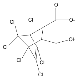
endosulfan γ-hydroxy carboxylate (ES HC)
