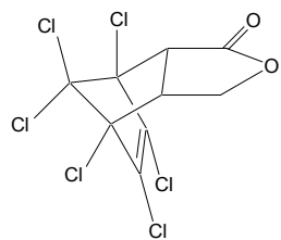
endosulfan lactone (ES lactone)
