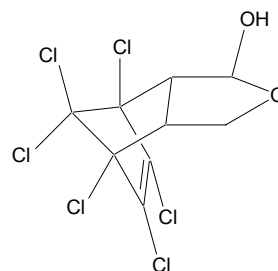
endosulfan α-hydroxyether (ES HE)
