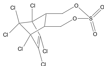
endosulfan sulfate (ES sulfate)
