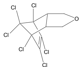
endosulfan ether (ES ether)
